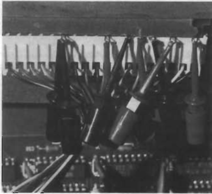
Figure 4: Added loops at keyboard connector and clip connections.
