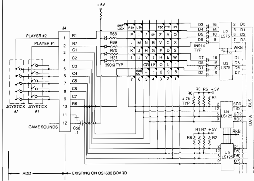
Figure 1: Keyboard/Joystick Schematic
