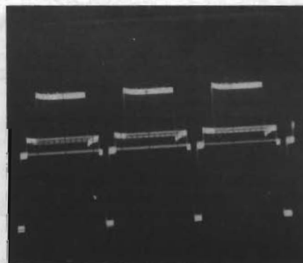
Photo 5: An oscilloscope trace of three lines of horizontal video.
