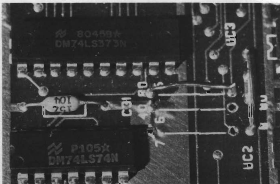
Figure 3: Detail showing jumpers 5, 6, 7, and 8.
